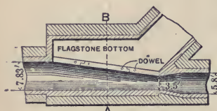
FIG. 3. STORM OVERFLOW, DENVER, COLO.
